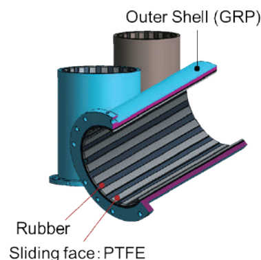
Sliding face: PTFE
