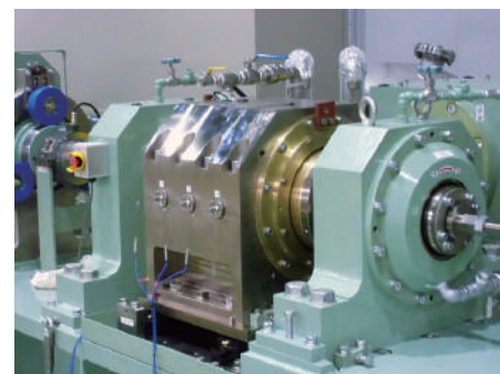
Test Equipment of 300mm shaft Dia.
